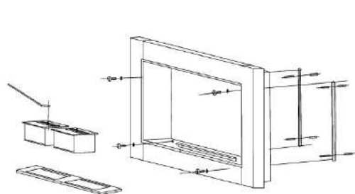
Wall Mounted
